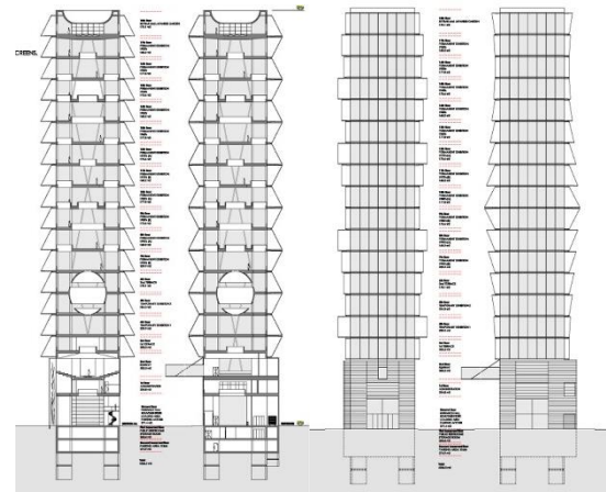
Figure 6: Transformer Tower, Sections and facade
