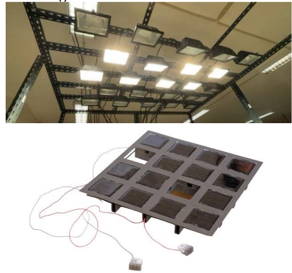
Figure 13: Greengrid prototype under solar simulator
