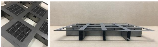
Figure 11: Greengrid prototype
