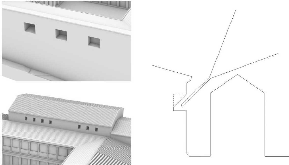
Fig. 14: Milling limitations
