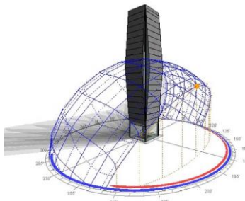
Figure 8: Solar Diagram
