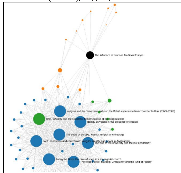
Abb. 6: Citation Graph
